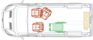
INTERNAL TRANSFER SEATING LAYOUT
