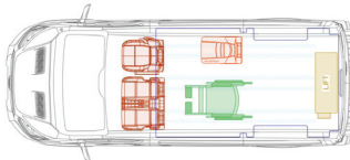
INTERNAL TRANSFER SEATING LAYOUT
